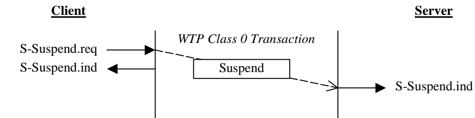
Figure 21. Session Suspend
